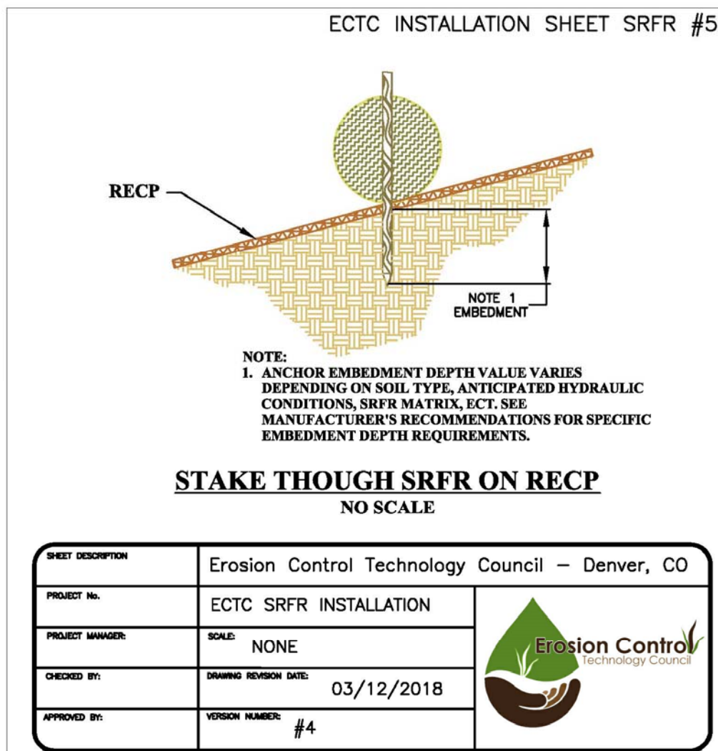
Figure 5 Stake through RECIP on top of RECIP/HECP.
