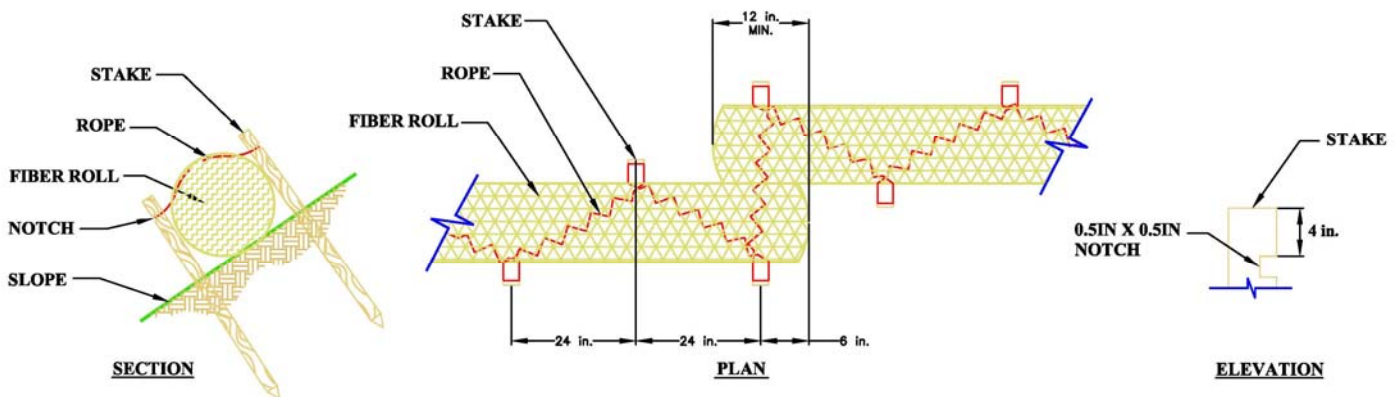
LASHED SRFR INSTALLATION DETAIL NO SCALE
